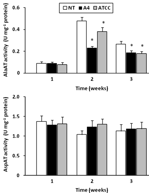
Fig. 5. Activity of alanine aminotransferase (AlaAT) and aspartate aminotransferase (AspAT) in hairy root clones of Physalis ixocarpa . Values are means of three independent experiments \pm SD. Statistically significant differences ( P < 0.05 ) between the A4 and ATCC clones and non-transformed roots (NT) are asterisked.
