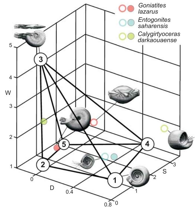
Fig. 8. Ammonoid morphospace after Tendler et al. (2015) using the Raupian parameters W (whorl expansion rate), S (shape of the generating curve), and D (distance between the generating curve and the coiling axis). Note that the juveniles (empty symbols) of Calygyrtoceras darkaouaense and Goniatites lazarus (in contrast to the respective adults) lie outside of the five-sided pyramid. Juvenile Nomismoceras sp. plots near vertex 1, Entogonites spp. between 1 and 4, and juvenile Bollandites sp. near 4. A Devonian pinacitid is depicted near vertex 3 to illustrate the conch morphology.
