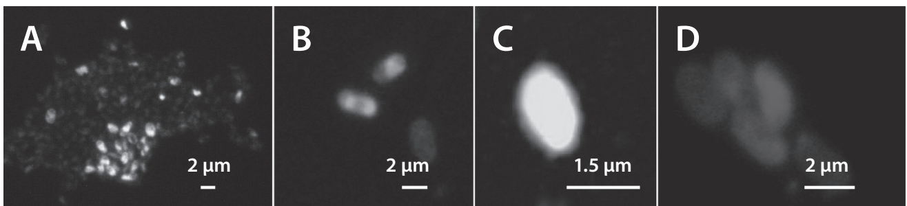
Figures 1A, B, C, D. Fluorescent in situ hybridization (FISH) images of spores of E. hellem (A), E. intestinalis (B), E. bienewsi (C), and E. cuniculi (D).
