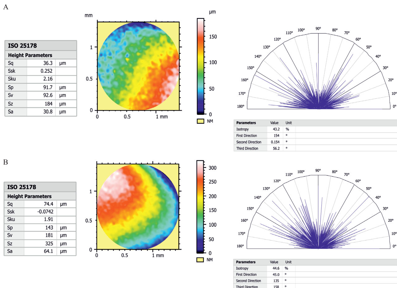
Fig. 2. Surface morphology characterization of ‘maize 1’ – statistic characteristics, 3D morphological views and polar graph with texture directions for: A – side ‘a’, position 1, B – side ‘b’, position 1.
