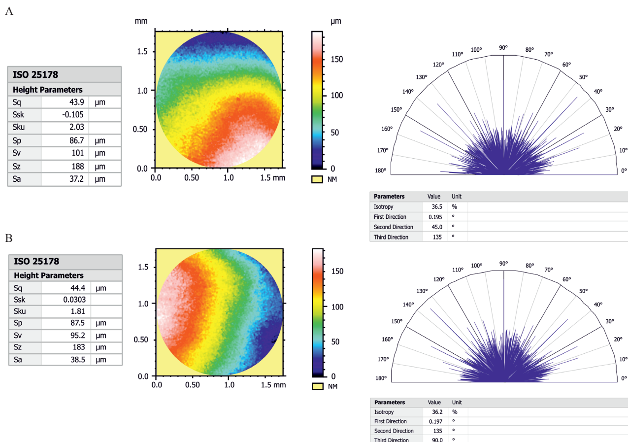
Fig. 3. Surface morphology characterization of ‘maize 2’ – statistic characteristics, 3D morphological views and polar graph with texture directions for: A – side ‘a’, position 1, B – side ‘b’, position 1.
