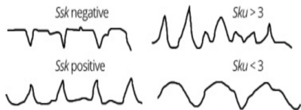
Fig. 6. Schematic representation of surfaces with different skewness (left) and kurtosis (right).
