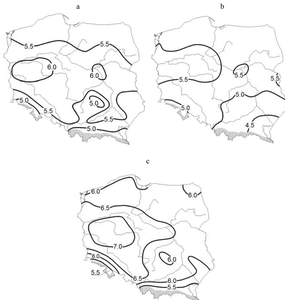
Fig. 7. Spatial distribution of the vapour pressure deficit (hPa) in the period Ee-H: a – average for the period 1966–2005, b – in 1974, c – in 1992
