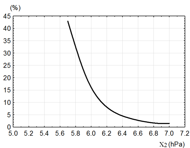
Fig. 4. Average national incidence of vapour pressure deficit \geq 5.7 hPa in the period Ee-H (%)
