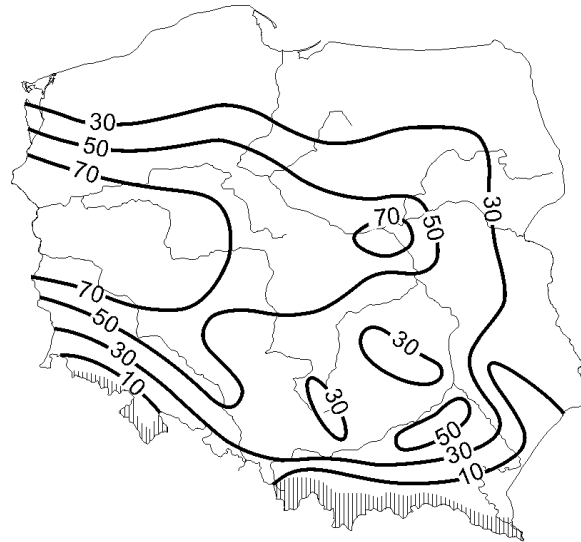
Fig. 5. Incidence of vapour pressure deficit \geq 5.7 hPa (%) in the period Ee–H (%)
