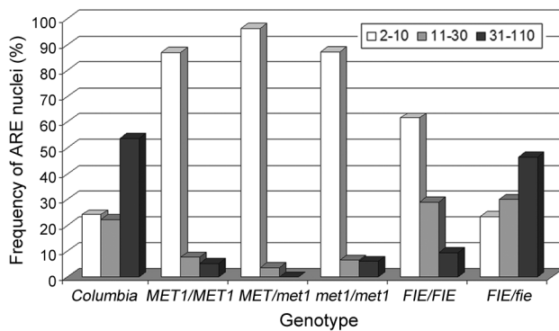
Fig. 5. The frequency of autonomous endosperm (AE) nuclei. Three developmental stages of free-nuclear AE were determined on the basis of AE nuclei number: 2–10, 11–30, 31–110.
