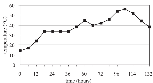
Fig. 1. Course of temperature during composting process.
