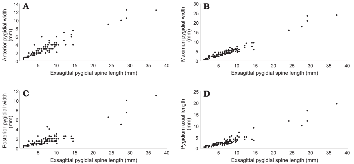
Fig. 18. Bivariate plot showing relationship between exsagittal pygidial spine length and the anterior pygidial width (n = 100) (A), maximum pygidial width (n = 107) (B), posterior pygidial width (n = 108) (C), and pygidium axial length (n = 108) (D) in paradoxidid trilobite Eccaparadoxides pradoanus (Verneuil and Barrande in Prado et al., 1860) from the Purujosa trilobite assemblage, Solenopleuropsis thoralis Biozone, middle Cambrian, Spain.
