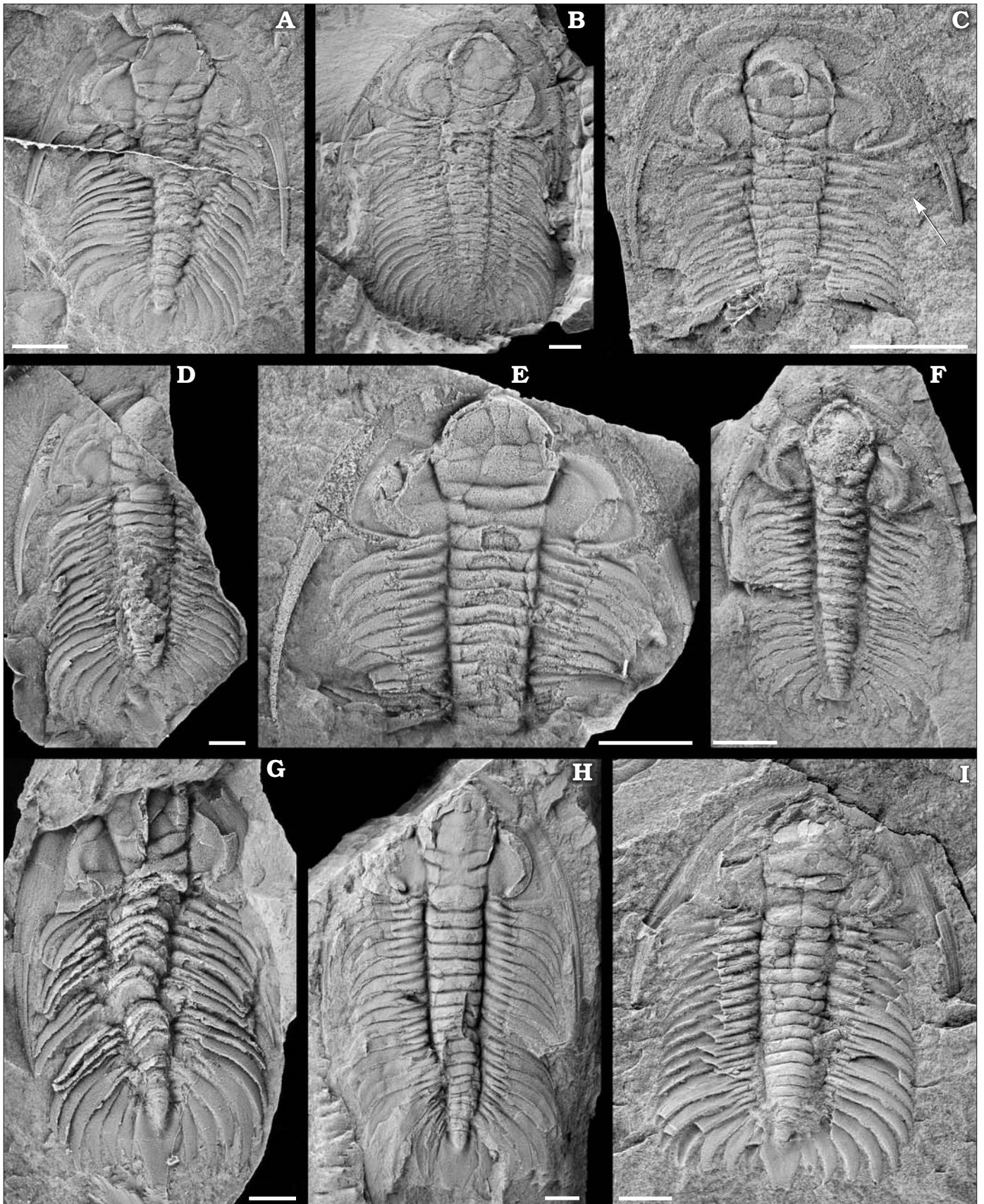
Fig. 5. Articulated specimens of paradoxidid trilobite Eccaparadoxides pradoanus (Verneuil and Barrande in Prado et al., 1860) with homonomous thorax, from the Purujosa trilobite assemblage, Solenopleuropsis thoralis Biozone, middle Cambrian, Spain with homonomous condition. A, C, E–G. Latex casts. A. MPZ2011/15. C. MPZ 2011/64, despite of small specimen size, the first two pleural spines are not macrospinous (arrow). D. MPZ2011/17. →
