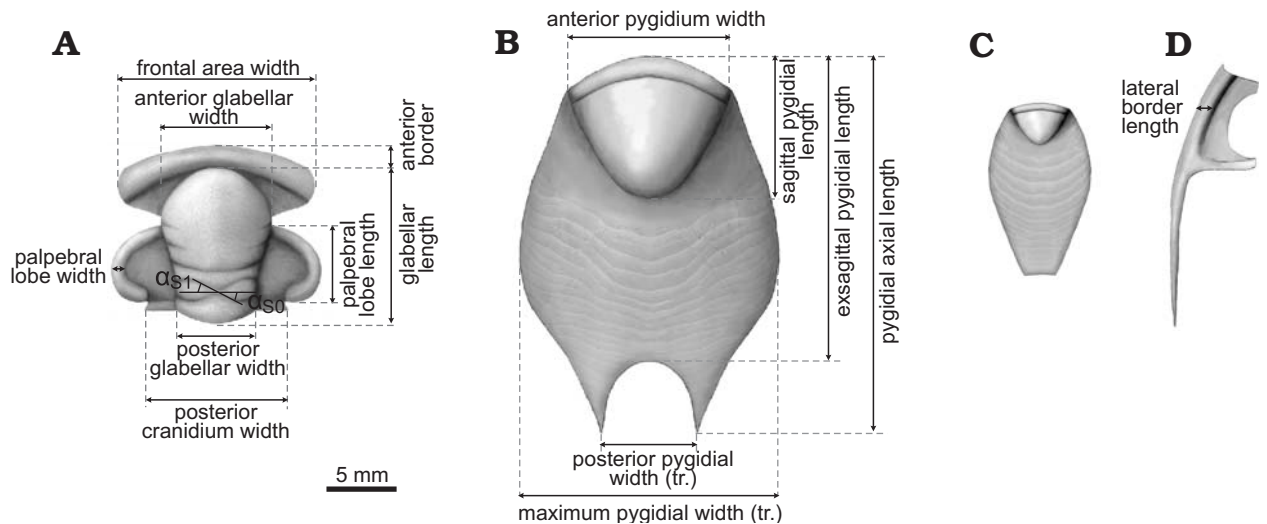
Fig. 2. Reconstruction of the cranium (A) and two types of pygidia of paradoxid trilobite Eccaparadoxides pradoanus (Verneuil and Barrande in Prado et al., 1860); with features measured on the dorsal view indicated type Eccaparadoxides mediterraneus (Pompeckj, 1901) pygidium (B) and type E. pradoanus (Verneuil and Barrande in Prado et al., 1860) pygidium (C), and reconstruction of the librigena (D). Abbreviations: \alpha_{s1} , angle of furrow 1; tr., transversal.
