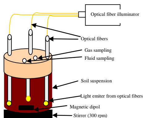
Fig. 1. Scheme of a single photoreactor equipped with optical fibres
