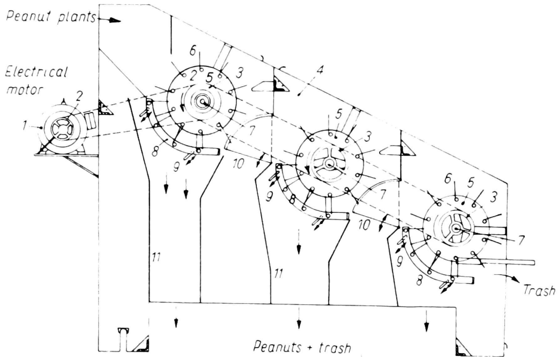
Fig. 1. Stationary mechanical picker, for laboratory tests
