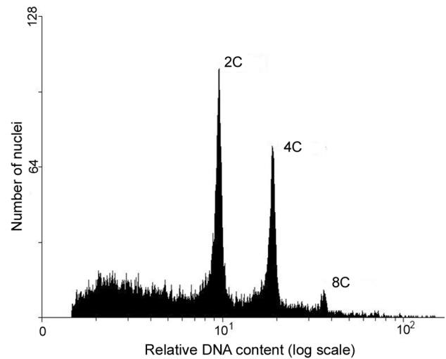
Fig. 1. Typical flow cytometry histogram for suspension of nuclei from T. repens inflorescence stalk.
