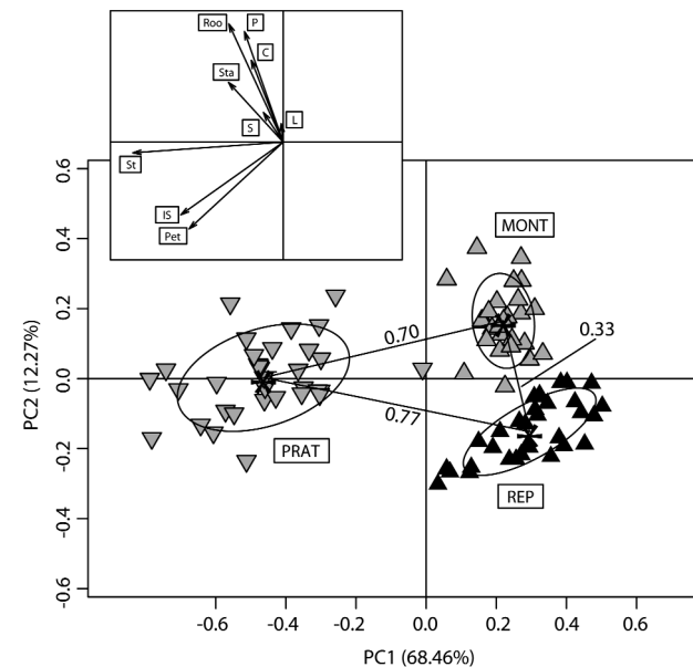
Fig. 3. Plot of eigenvalues of 92 individuals of T. pratense (PRAT), T. repens (REP) and T. montanum (MONT) by principal component analysis. Euclidean distances of group centroids (asterisked) were calculated. Eigenvectors of organs given in inset. Roo – root; St – stem; Pet – petiole; L – leaf; IS – inflorescence stalk; S – sepal; P – petal; Sta – stamen; C – carpel.
