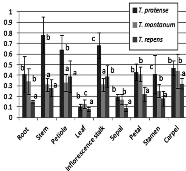
Fig. 2. Cycle values of organs in T. pratense , T. montanum and T. repens . Bars represent mean cycle values. Data are means \pm SD. Organs with cycle value < 0.1 are nonendopolyploid. Differences in endopolyploidy level between species for each organ tested by ANOVA (log10-transformed data, P < 0.05 ). Homogeneous groups were separated by Tukey's HSD test. Identical letters designate organs whose mean cycle values do not significantly differ at P < 0.05 and which belong to the same group for that organ. Data for T. pratense taken from Kocová and Mártonfi (2011).
