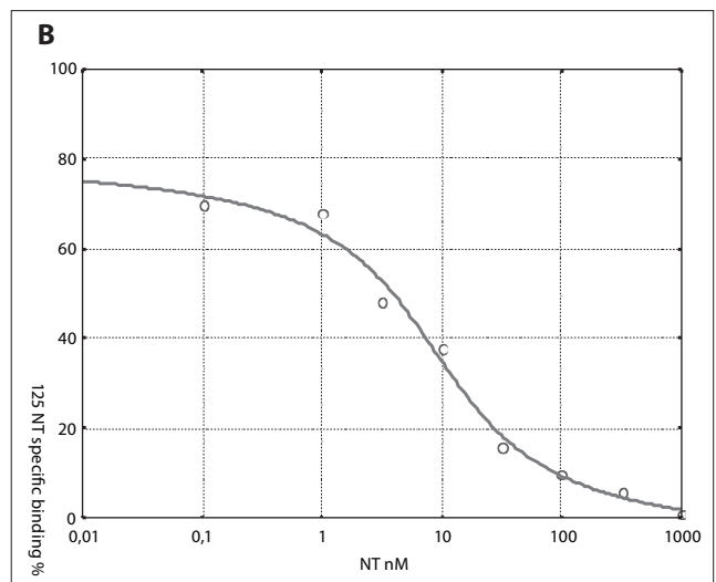
Figure 3 A). Scatchard analysis B). Inhibition of specific binding of ^{125}\text{I} -NT to cell membrane hepatocytes of rats given in vivo Trp-NT one hour before sampling tissues in the dose of 15 nmol/kg b.m. Reported values are the means of three independent experiments performed in triplicate and variations did not exceed 5%
