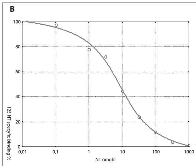
Figure 2 A). Scatchard analysis B). Inhibition of specific binding of ^{125}\text{I} -NT to cell membrane hepatocytes of rats given in vivo SR 48692 1 h before tissue sampling at the dose of 0.4 mg/kg b.m. Reported values are the means of 3 independent experiments performed in triplicate; variations did not exceed 5%
