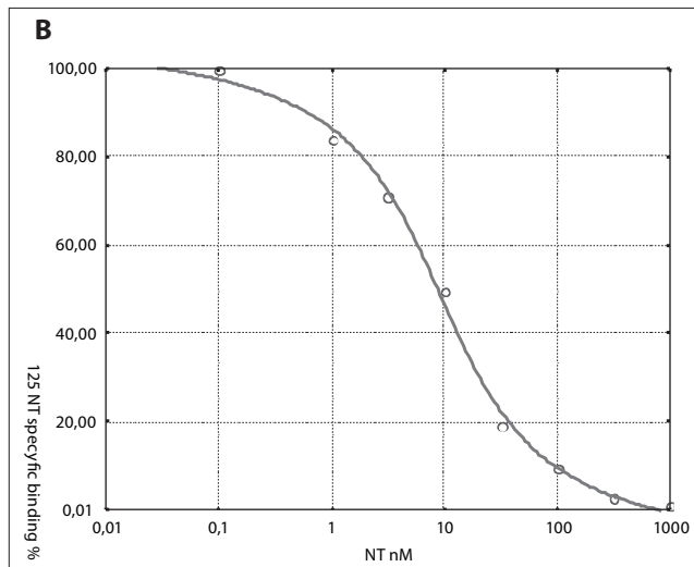
Figure 1 A). Scatchard analysis B). Inhibition of specific binding of ^{125}\text{I} -NT to cell membrane hepatocytes of rats given in vivo 0.9% NaCl 1 h before tissue sampling. Reported values are the means of 3 independent experiments performed in triplicate; variations did not exceed 5%
