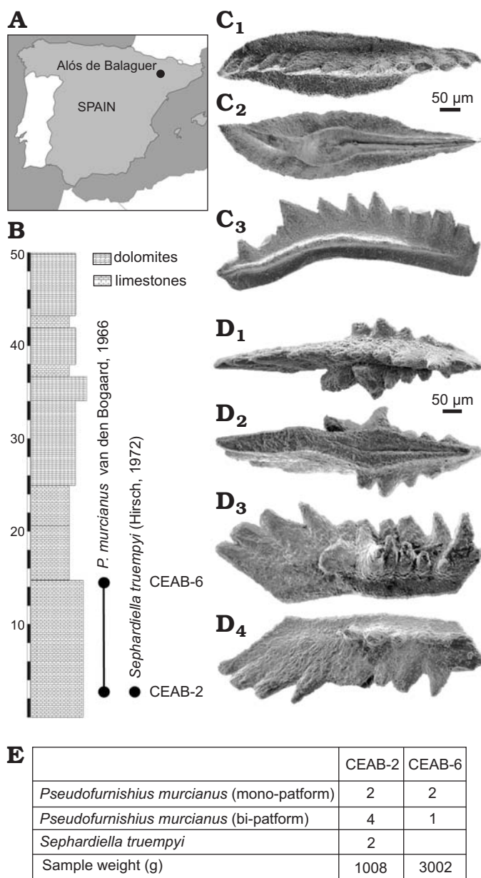
Fig. 7. A. Geographic location of Alós de Balaguer. B. Stratigraphic position of gondolellid conodonts in the Ladinian (Fassanian), Grey Limestone Unit, Pyrenees. C. Sephardiella truempyi (Hirsch, 1972), right element, MGUV-10407, sample CEAB-2, in occlusal (C 1 ), basal (C 2 ), and caudal (C 3 ) views. D. Pseudofurnishius murcianus Van den Boogaard, 1966, right element, MGUV-10105, sample CEAB-2, in occlusal (D 1 ), basal (D 2 ), caudal (D 3 ), and rostral (D 4 ) views. E. Conodont distribution at Alós de Balaguer.
