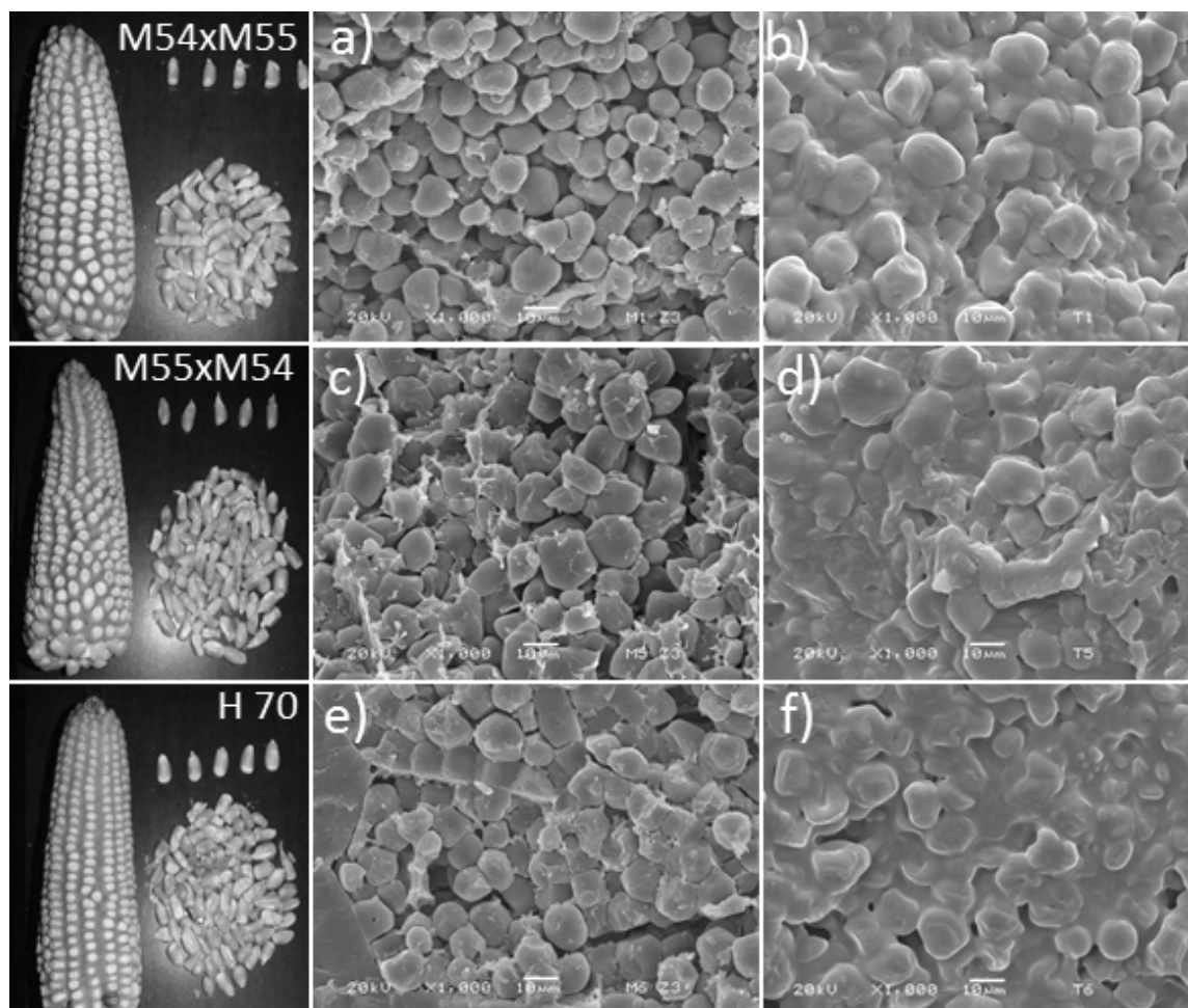
Fig. 5. SEM images 1000x: M54xM55 a – maize, b – tortilla; M55xM54 c – maize, d – tortilla; H-70 e – maize, f – tortilla.
