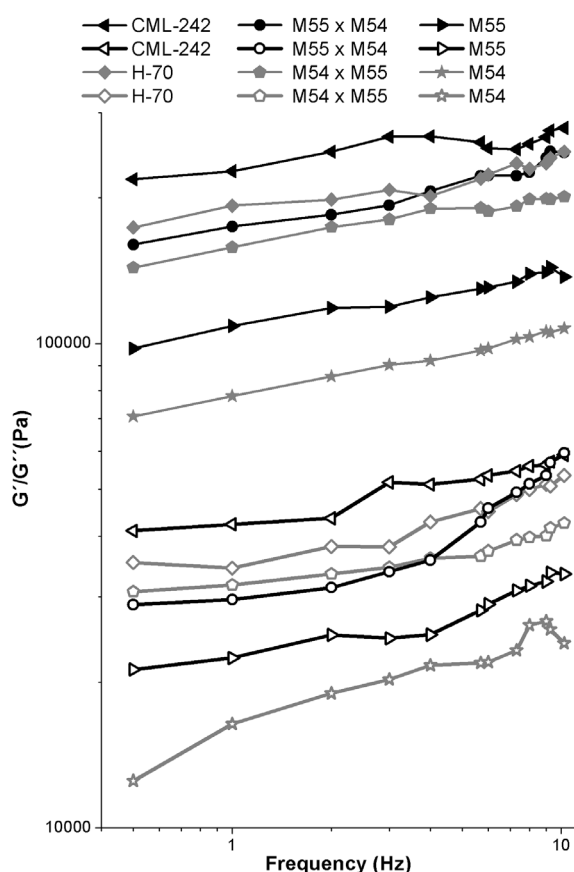
Fig. 2. Viscoelastic properties of masa obtained from six maize genotypes. Filled symbols correspond to G' and empty symbols to G'' .
