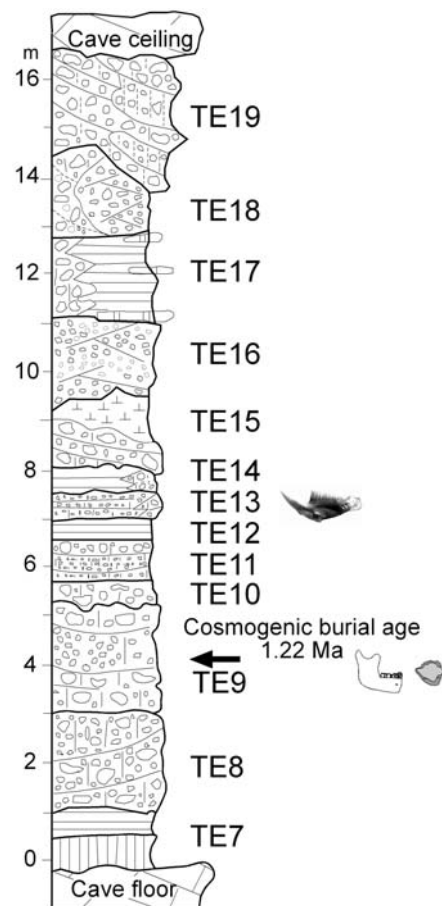
Fig. 3. Synthetic column showing the lithostratigraphic units of the north section of the Sima del Elefante site, labelled TE (levels TE7 to TE19). Levels that correspond to the Lower Red Unit, TE-LRU are TE7 to TE14. Units TE20 to TE22 do not outcrop here, but in the southern section (see Fig. 2). Black arrow points to level TE9 from which the recently discovered human remains were retrieved, and where the burial dating, based on the radioactive decay of cosmogenics, has been calculated (Carbonell et al. 2008). The small arvicoline mandible points to the level (TE13) where the holotype of Arvicola jacobaeus sp. nov. was found. The figure has been modified from Carbonell et al. (2008).
