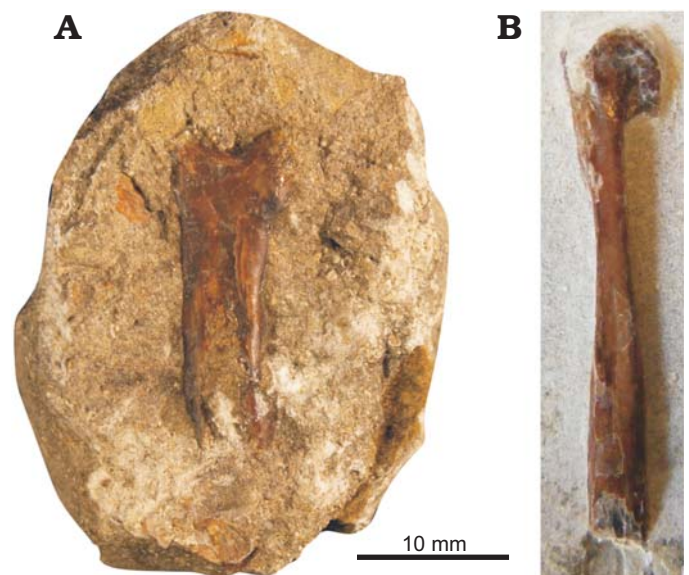
Fig. 8. Metacarpals from the Great Oolite Group from Taynton Limestone Formation (Bathonian, Middle Jurassic), Stonesfield, Oxfordshire, UK. A. A non-monofenestratan pterosaur indet. (MUM STR1244b), left MCIV in anteroposterior view. B. ?Monofenestrata indet. (NHMUK PV R 28160b), right? MCIV in dorsoventral view.
