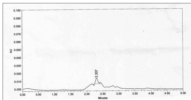
Figure 4 Chromatogram after treatment with 1% H 2 O 2 (Pure DOX, 200 µg/mL).
