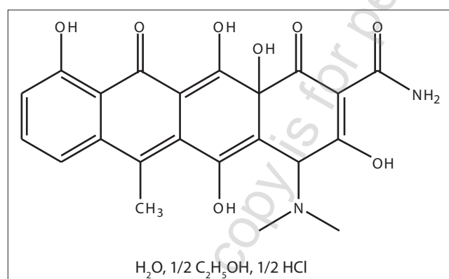
Figure 1 Structure of doxycycline hyclate.
