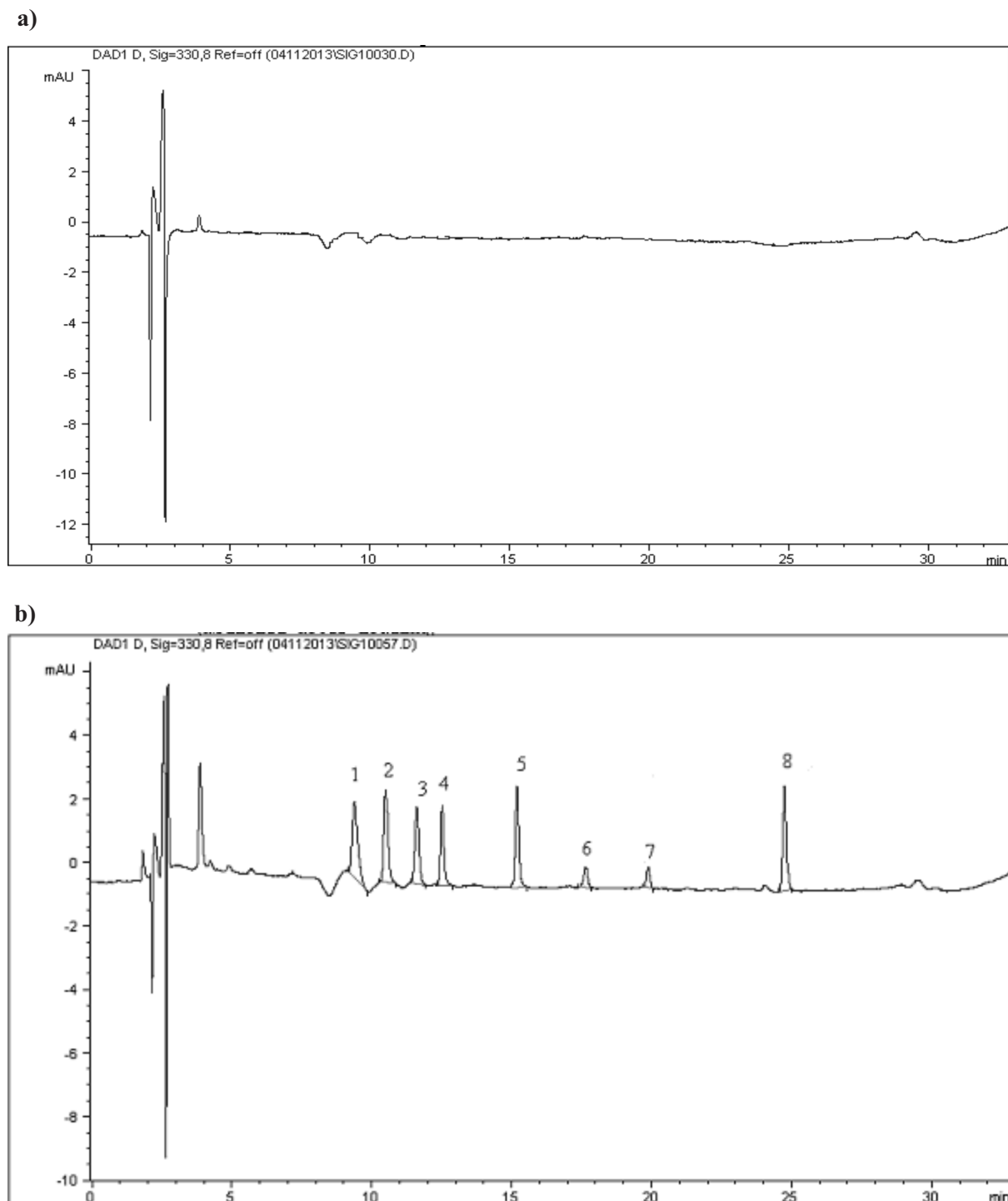
Fig. 1. Representative chromatograms of (a) blank water sample and (b) water sample spiked with mixture of oxytetracycline (1), ciprofloxacin (2), tetracycline (3), enrofloxacin (4), sarafloxacin (5), chlortetracycline (6), doxycycline (7), flumequine (8), at a concentration of 10 \mu\text{g/L} .
